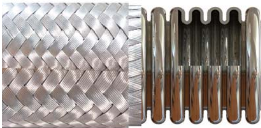
Annular profile Corrugations Independent corrugations straight & parallel
