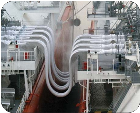
Ship to shore transfer of Liquefied Natural Gas (LNG)
